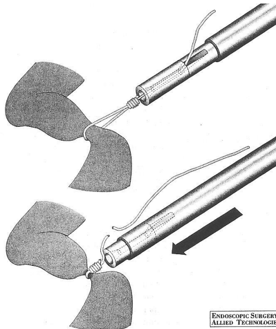
Figure 3: The "cutting knot pusher" entails an outer sleeve which permits exact cutting of the thread subsequent to pushing down and tightening of an external slip knot.
